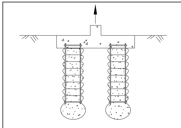
Figure 4. Geopier Elements with Uplift Harnesses
